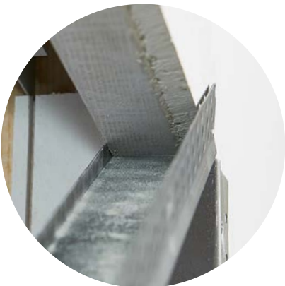
4. Cut the Metal Trim to the opening width and slide over the Timber Trim and plasterboard and fix into place.
